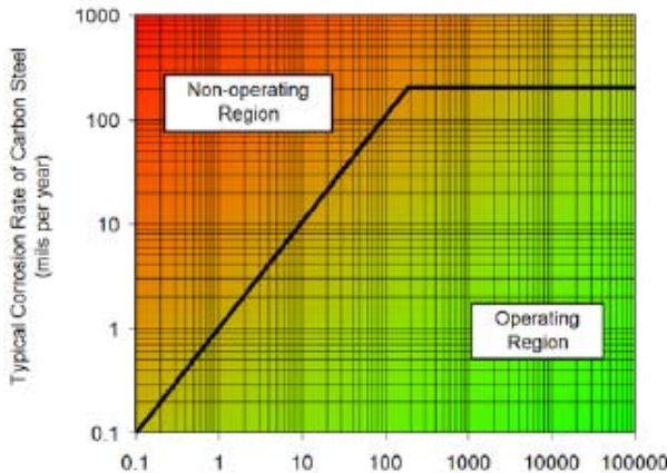
Operating Range for Model 9020
