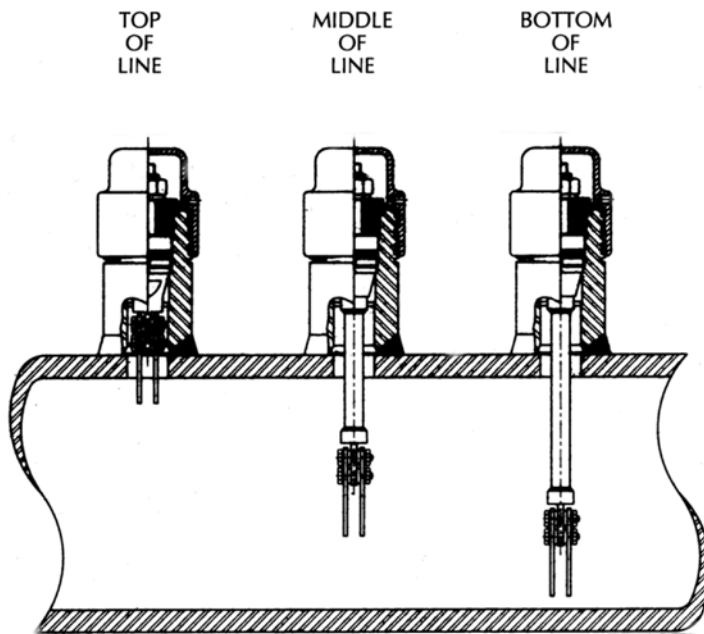
FIG. 1 Coupons shown rotated 90° from normal position.
