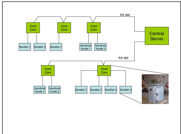
CORD-COM Remote CP Monitoring with ICMS3
