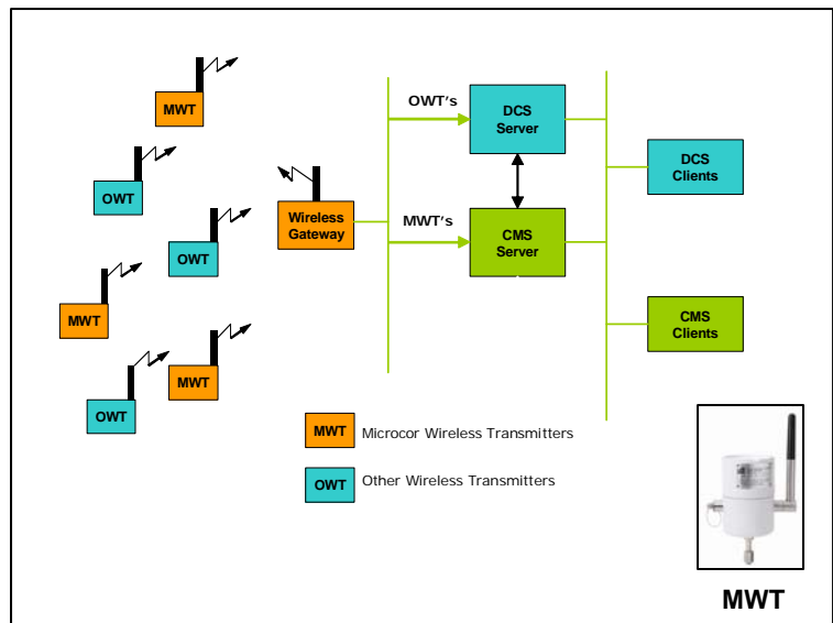
New Wireless Transmitters can be fed Directly into ICMS3
