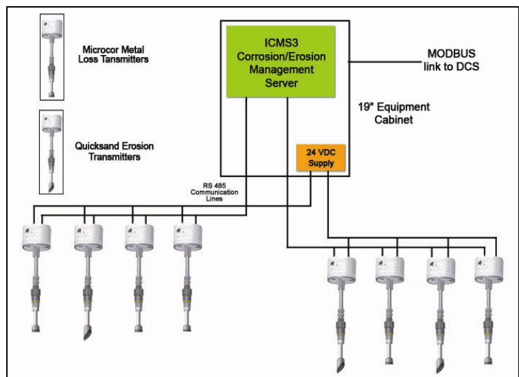
ICMS3 System shown with Microcor & Quicksand Transmitters
