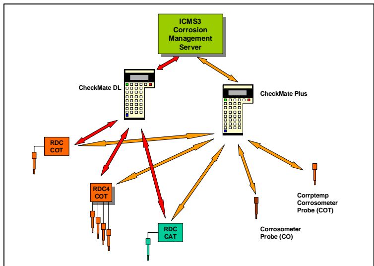
Data can be collected and transferred to the ICMS3 System using Corrdata Data-Loggers
