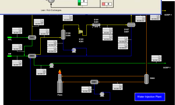
Typical Mimic Diagrams
