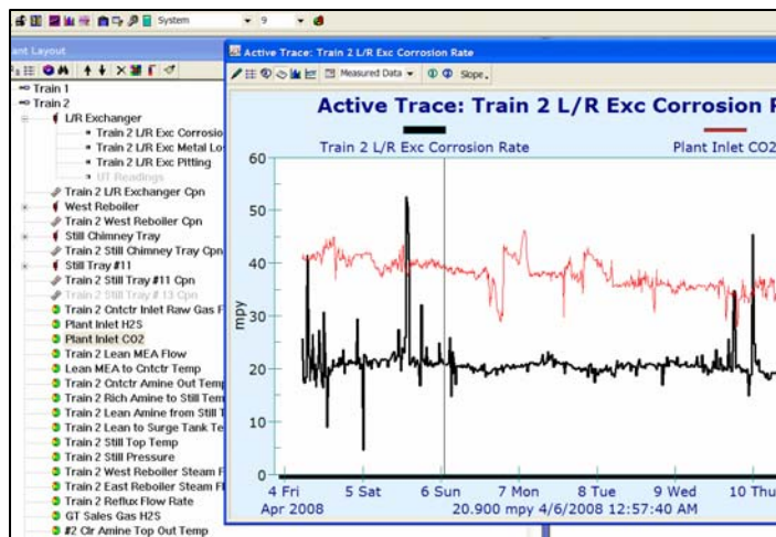
Metal Loss Graph
