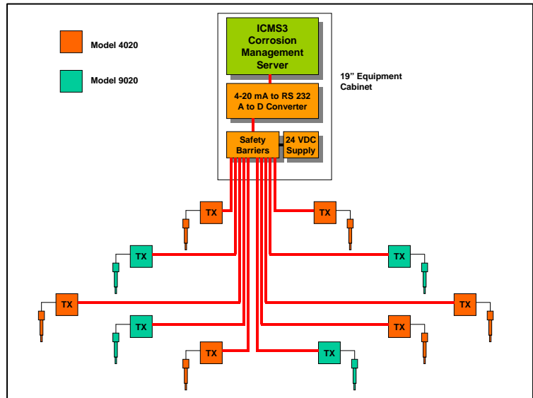
ICMS3 Server shown with Analog to Digital Converter
