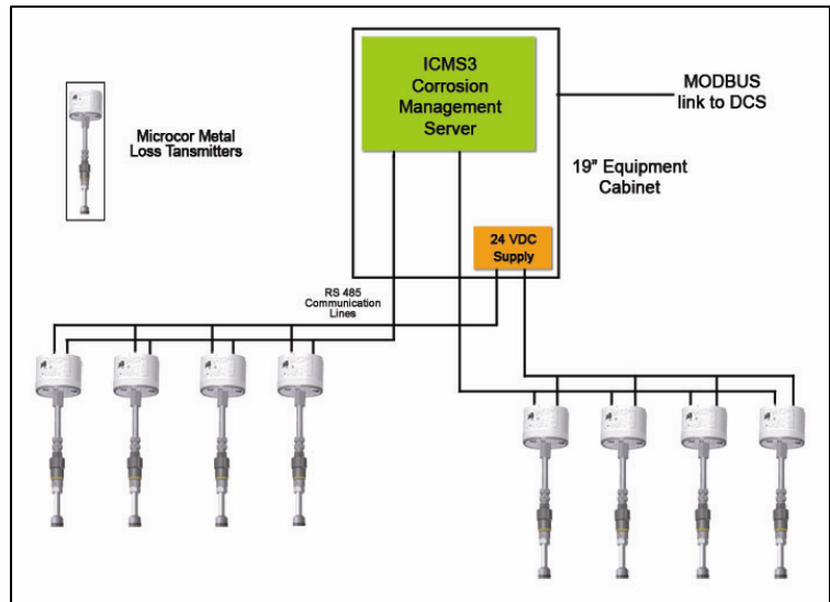
Simple Wired System with Microcor Transmitters
