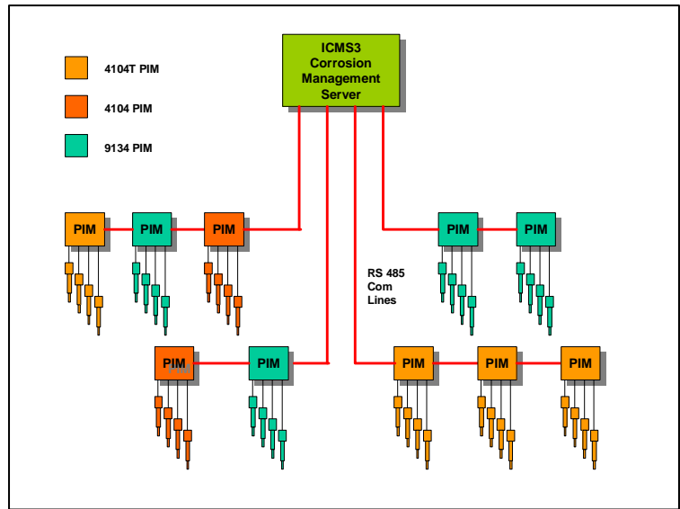
ICMS3 shown with Probe Interface Modules
