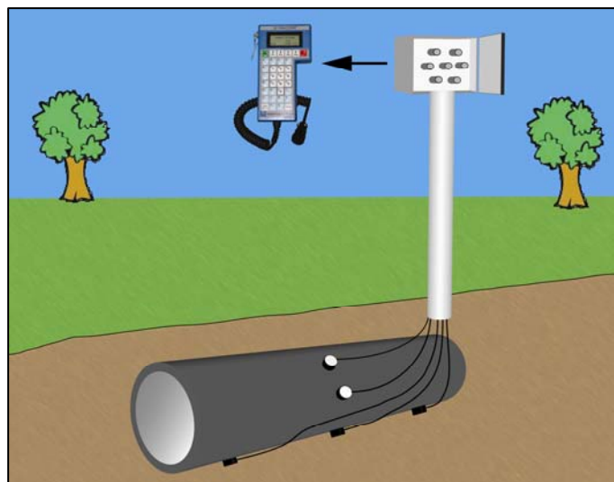
Ultracorr transducers are connected to a junction box at one central location for data collection
