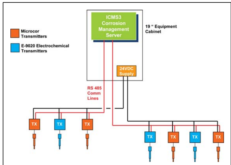
ICMS3 System shown with Microcor & E-9020 Transmitters
